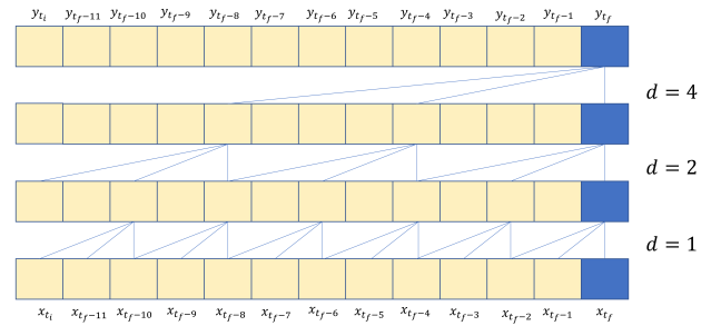
Figure 2: TCN architecture
